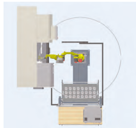
Configuration - Parallel Front Entry
