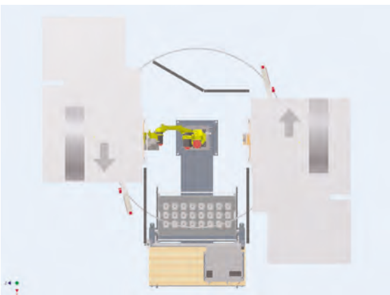
Configuration - Dual Machine Parallel Side Entry
