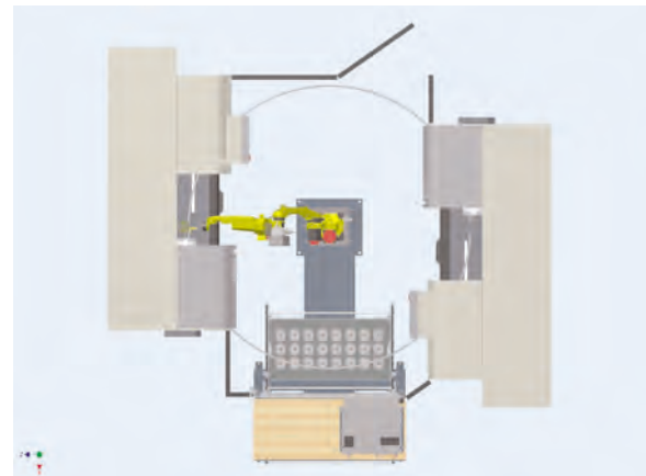
Configuration - Dual Machine Parallel Front entry
